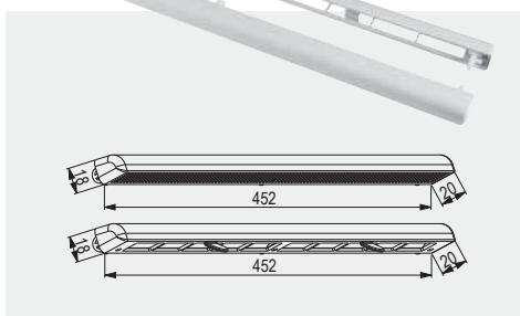
Slimline 4000
